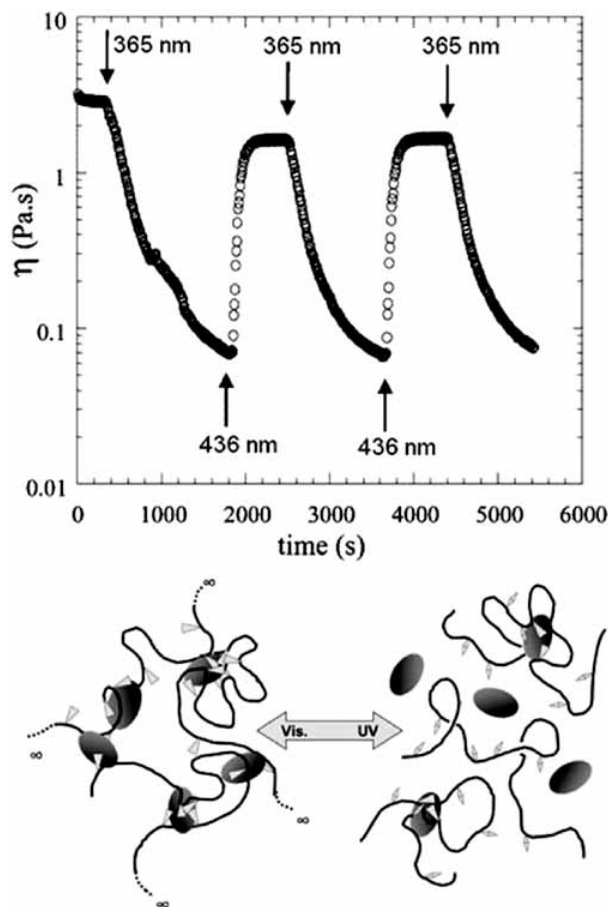
Fig. (7). Variation of viscosity of 1 wt % azobenzene copolymer solution (225-2C12Azo) in the presence of 0.7% bovine serum albumin, under exposure to light with alternating the wavelength between UV (365 nm) and visible (436 nm). Initially, the sample was equilibrated for 24 h in the dark (all- trans form) and first exposed to UV at time 400 s. The sketch of light-triggered binding of proteins on the azobenzene copolymer shown below indicates that proteins are mostly bound under exposure to visible light and that are released under UV exposure. The trans -azobenzene side groups are drawn as triangles, and their cis form appears as mostly unbound lozenges. Reprinted in part with permission from [64]. Copyright (2006) American Chemical Society.
