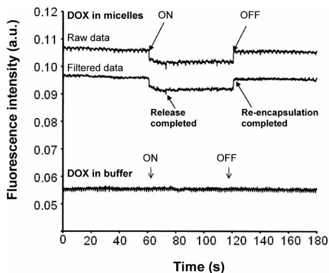
Fig. (8). Example of release profiles of doxorubicine (DOX) from a 10% Pluronic solution and from phosphate buffer. DOX concentration 6.7 \mu\text{g/ml} . Raw and Fourier-filtered data are presented for the 10% Pluronic solution. For the PBS solution, ultrasound was turned on at 60 s and off at 120 s; there was a negligible change of DOX fluorescence under sonication. Reprinted from [69] with permission from Elsevier.
